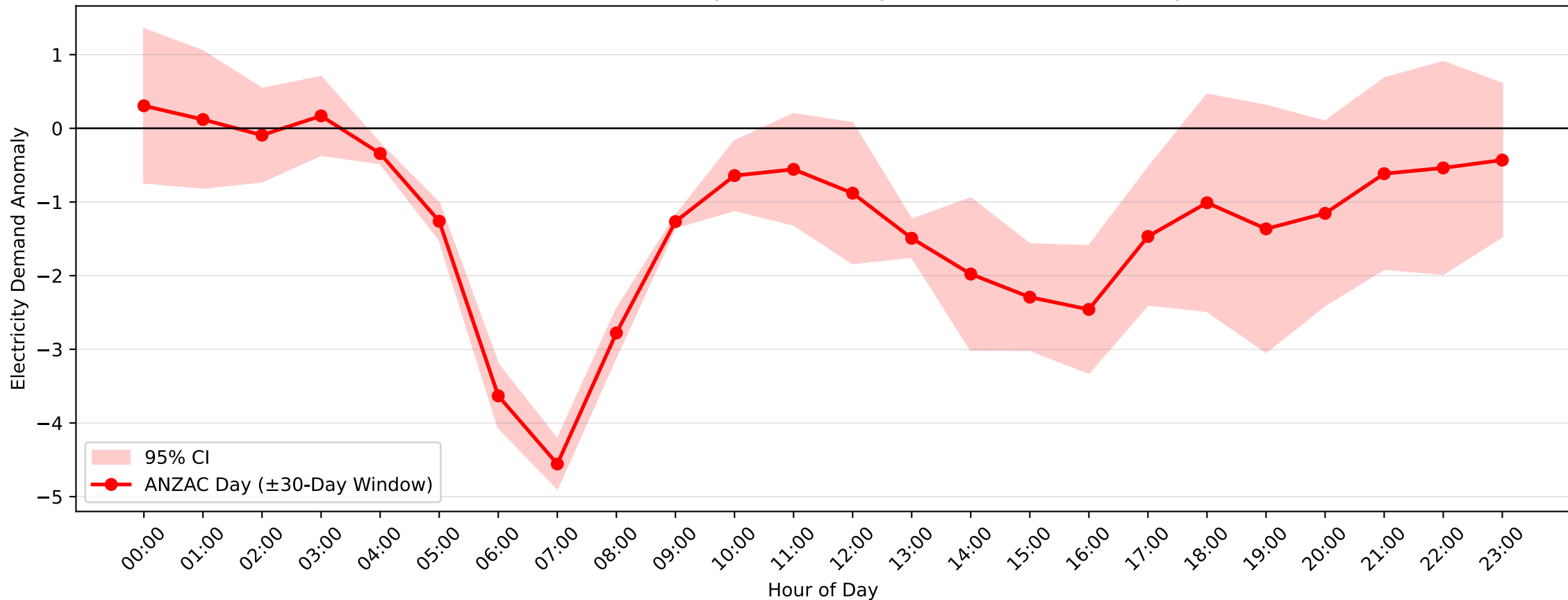
Dulwich Hill Demand Anomaly: ANZAC Day (2012–2013, \pm 30 -Day Window)
