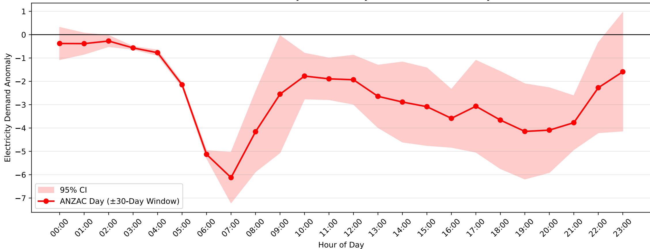
Dulwich Hill Demand Anomaly: ANZAC Day (2009–2010, \pm 30 -Day Window)
